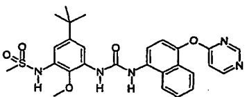
N-(5-tert-Butyl-2-methoxy-3-{3-[4-(pyrimidin-4-yloxy)-naphthalen-1-yl]-ureido}-phenyl)-methanesulfonamide;
